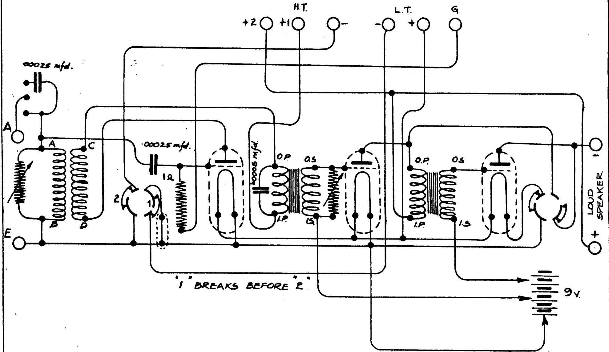
schematic Diagram of RECEIVER Type 31.
